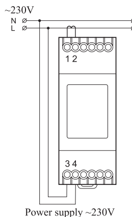
Connection diagram
